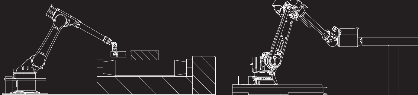
PolyMARK B Automatic cell for casting products hot marking
