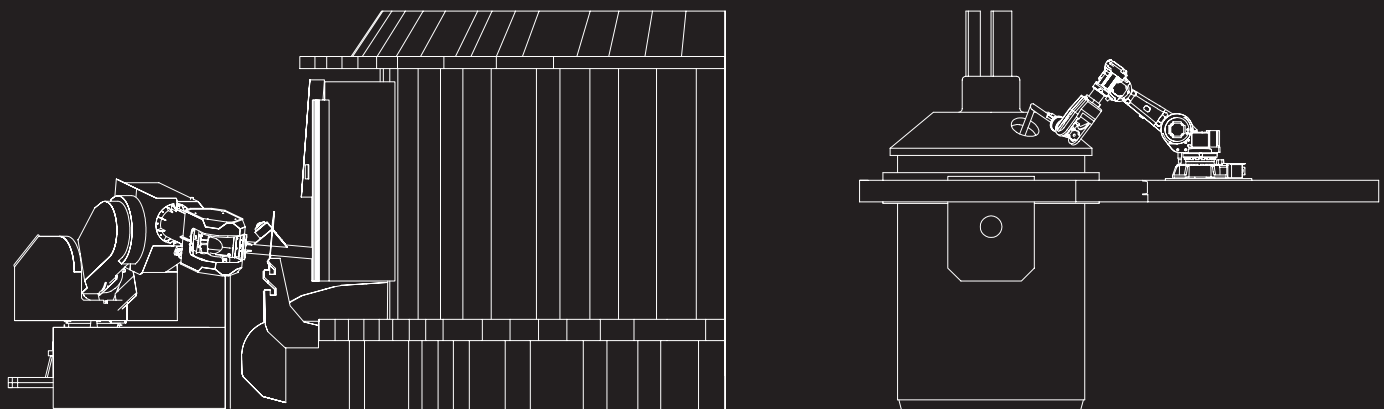
PolySAPLE EAF Automatic cell for EAF sample and measurement
